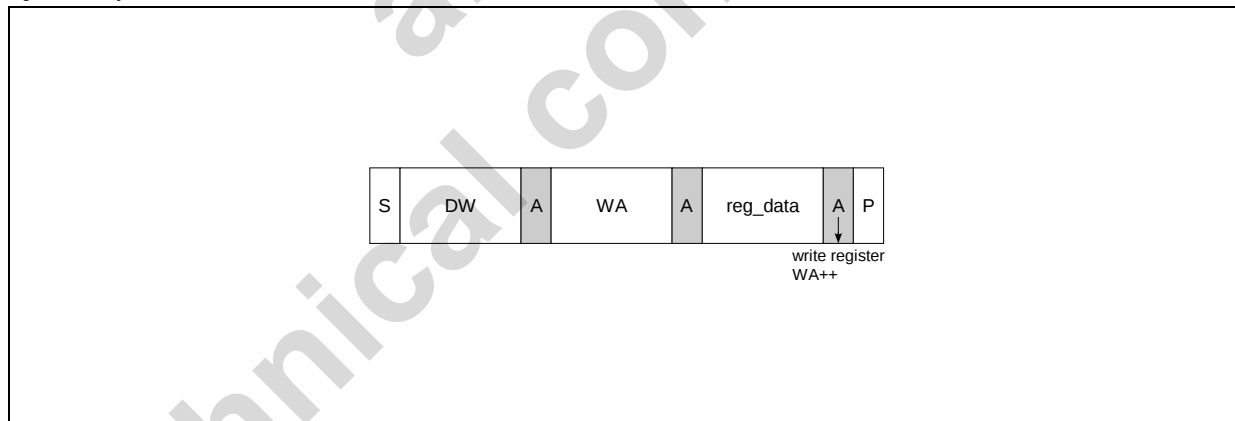
Figure 15. Byte Write
