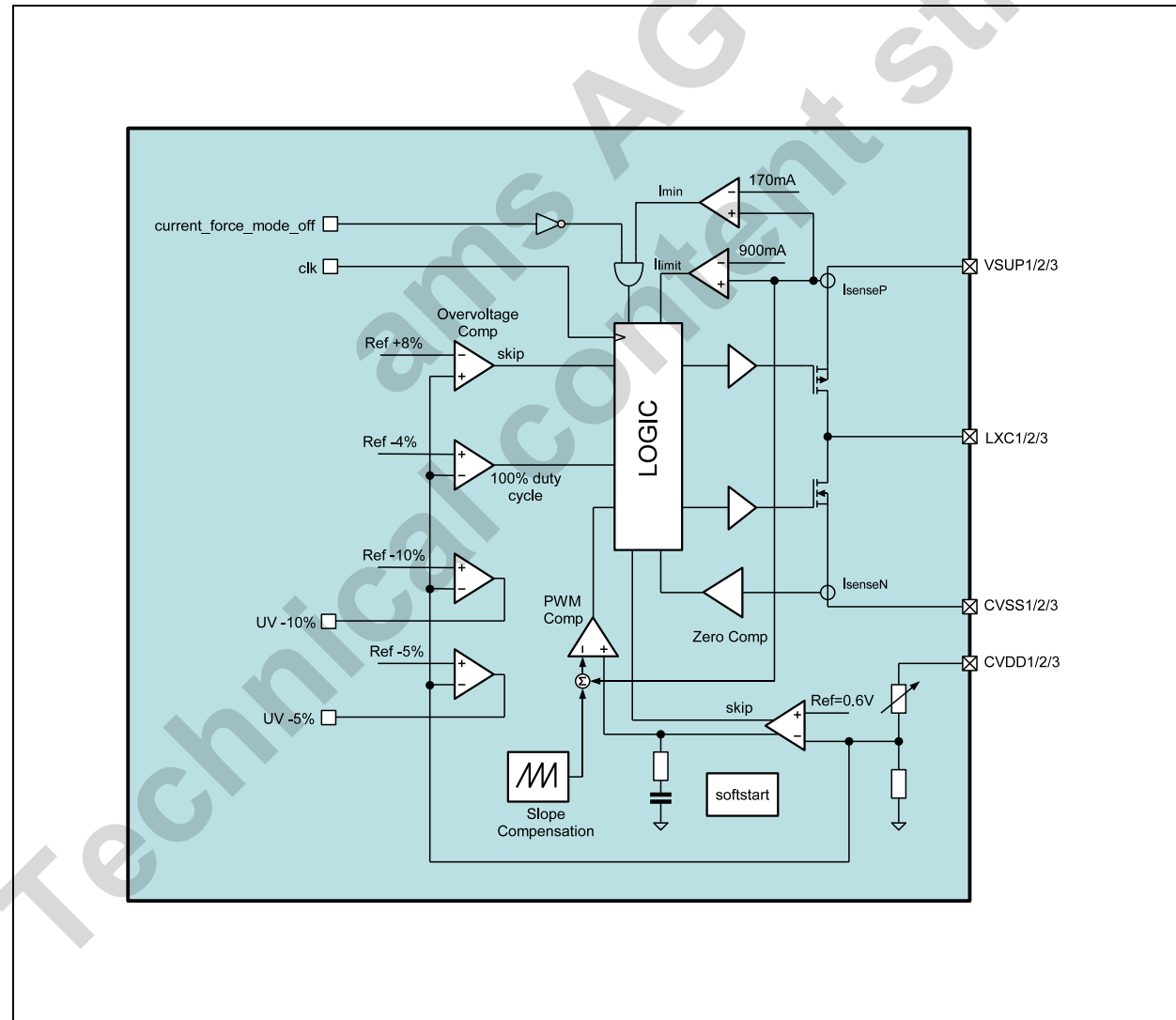
Figure 6. DCDC Step-Down Block Diagram
