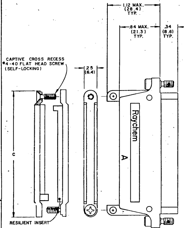
2 CABLE CLAMP (2-PIECE)
