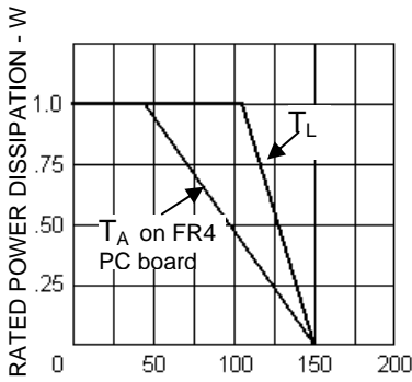
T_L , LEAD TEMP. ( ^{\circ}\text{C} ) 3/8" from body or T_A on FR4 PC Board
