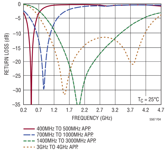
Figure 4. RF Input Return Loss
