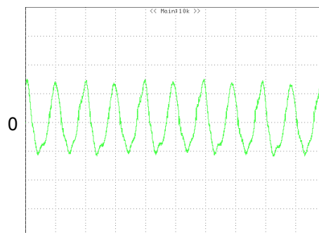
Figure 11: Input Terminal Ripple Current, i_c , at full rated output current and nominal input voltage with 12 \mu H source impedance and 100 \mu F electrolytic capacitor (200 mA/div, 2 \mu s/div)
