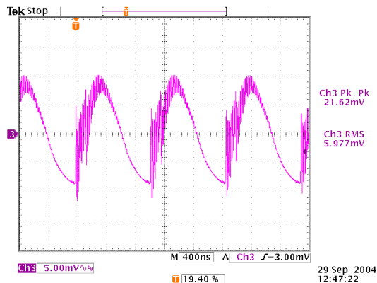
Figure 40. Output Voltage Noise, Full Load, No Interleave
