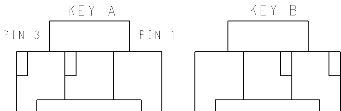
1*3 POSITIONS
