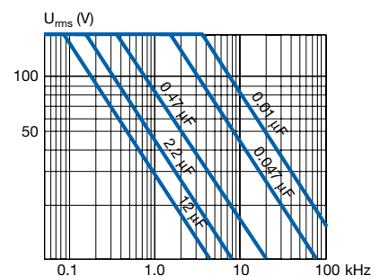
MMK7.5 ... 37.5 250/160
