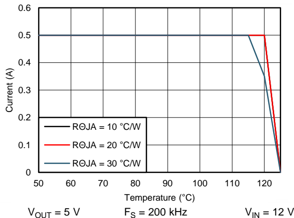
Figure 70. Derating Curve
