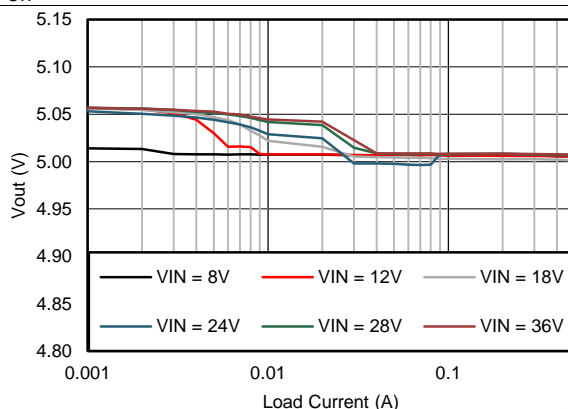
Figure 8. V_{OUT} Regulation
