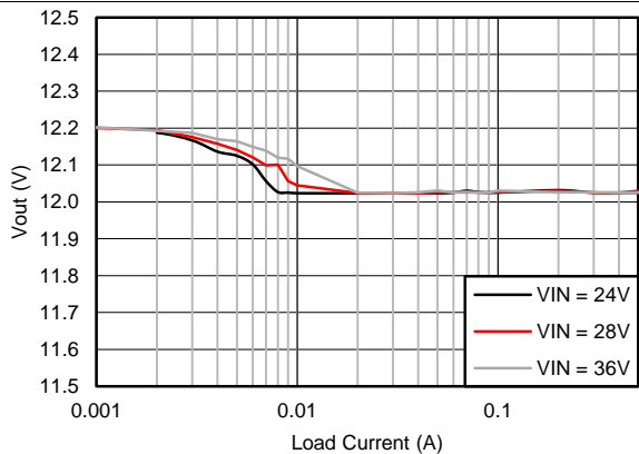
Figure 9. V_{OUT} Regulation
