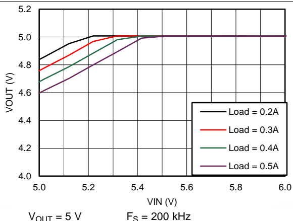
Figure 68. Dropout Curve
