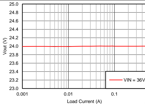
Figure 10. V_{OUT} Regulation
