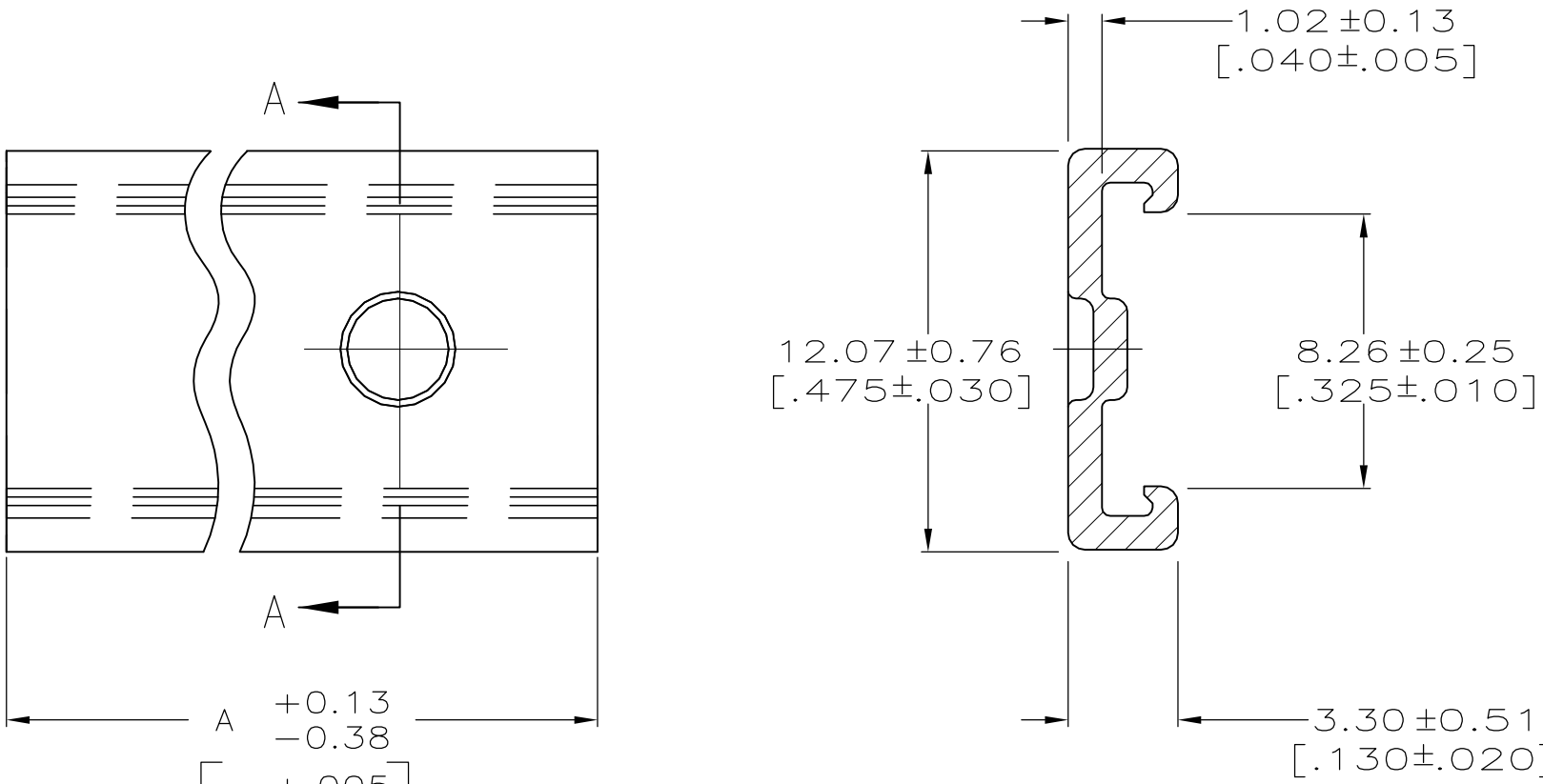
SECTION A—A
