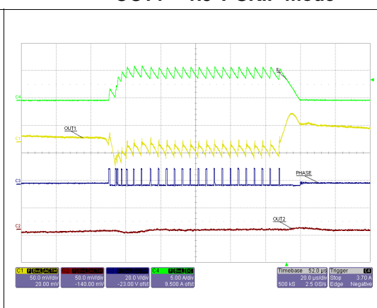
Figure 39. Load transient 0-5 A 2 A/ \mu s OUT1 = 1.5 V SKIP mode
