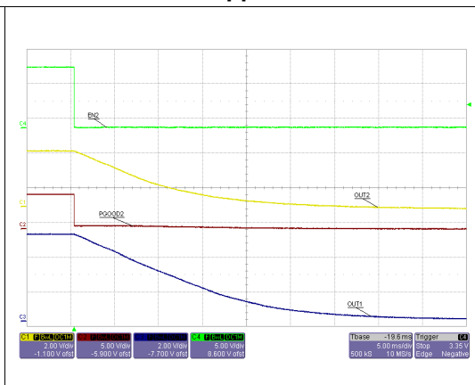
Figure 35. Soft-end, EN1=VREF2 no loads applied
