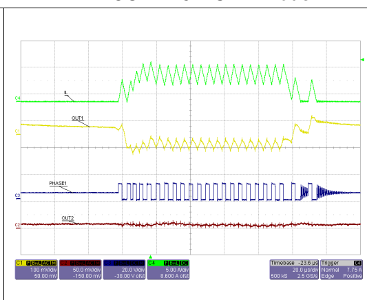
Figure 37. Load transient 0-5 A 2 A/ \mu s OUT1 = 5 V SKIP mode
