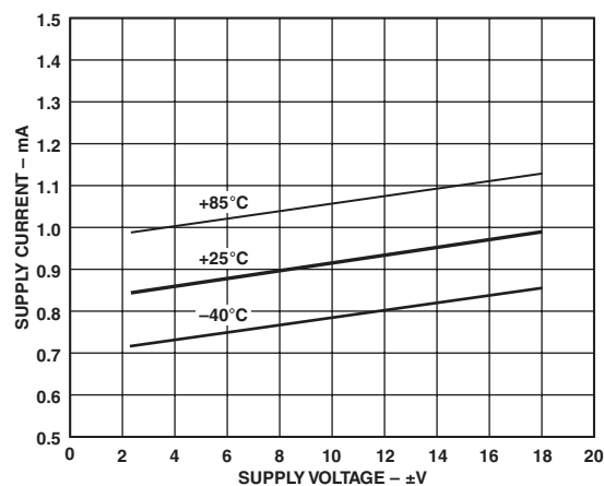
TPC 24. I_{\text{SUPPLY}} vs. V_{\text{SUPPLY}} and Temperature
