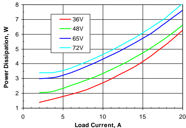
Figure 4: Power dissipation vs. load current and input voltage for SSQE48T20033 converter mounted vertically with air flowing from pin 1 to pin 3 at a rate of 300 LFM (1.5 m/s) and T_a = 25^\circ\text{C} .
