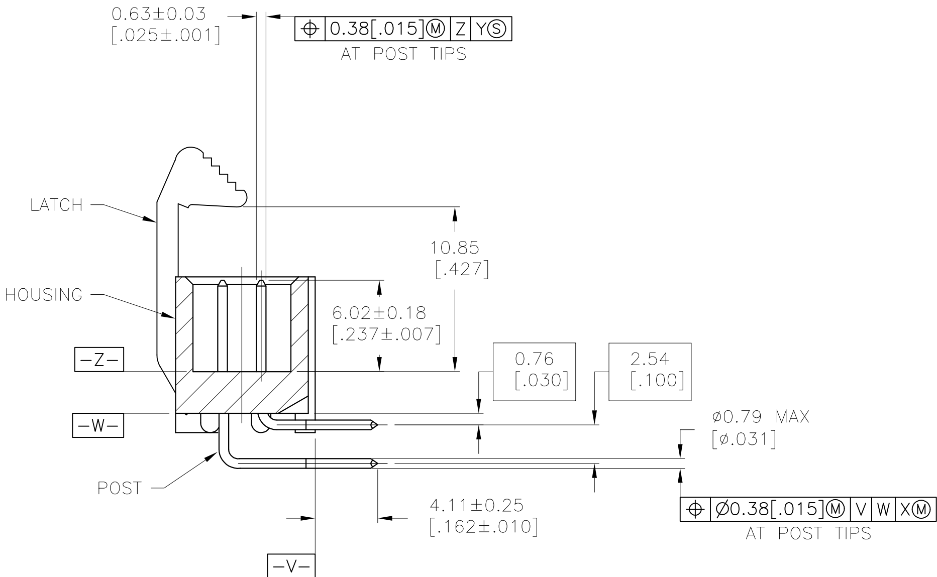
SECTION U-U
