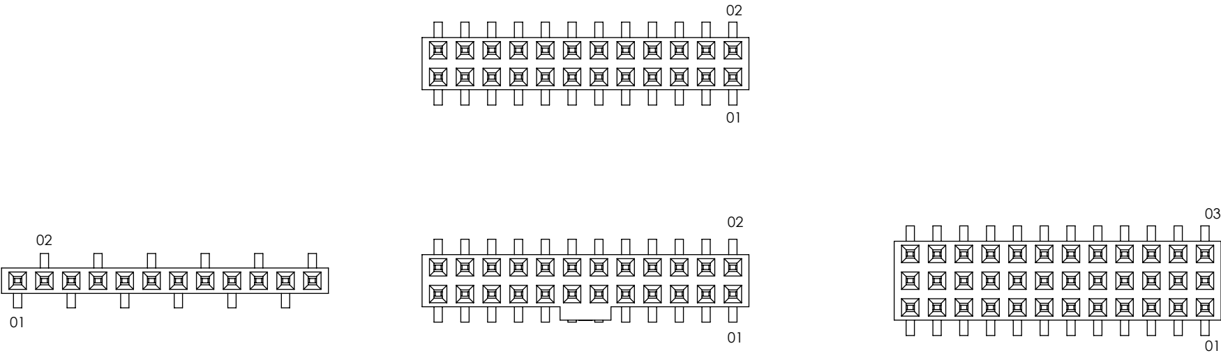
FIG 4 POLARIZATION LOCATION INSERT PK-06-N INTO SPECIFIED POS AND BREAK OFF TAB
