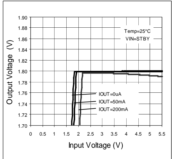
Figure 4. Line Regulation
