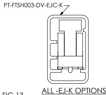
FIG 13 TUBE VIEWS
