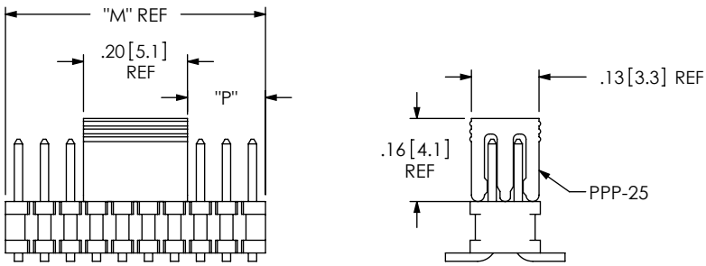
FIG 11 -P OPTION (DIFFERENT AS SHOWN, OTHERWISE SAME AS FIG 1)
