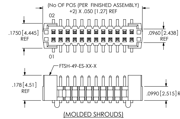
FIG 6 -ES OPTION (DIFFERENT AS SHOWN, OTHERWISE SAME AS FIG 1) (USE -02 OR -03 LEAD STYLE ONLY) (9 POS MIN FOR SNAP SHROUDS) (5 POS MIN FOR MOLDED SHROUDS)
