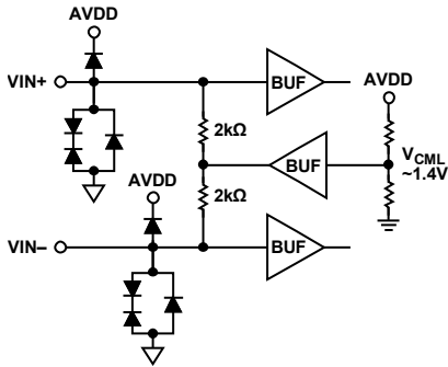
Figure 6. Analog Inputs ( V_{CM1} \sim 1.4V )
