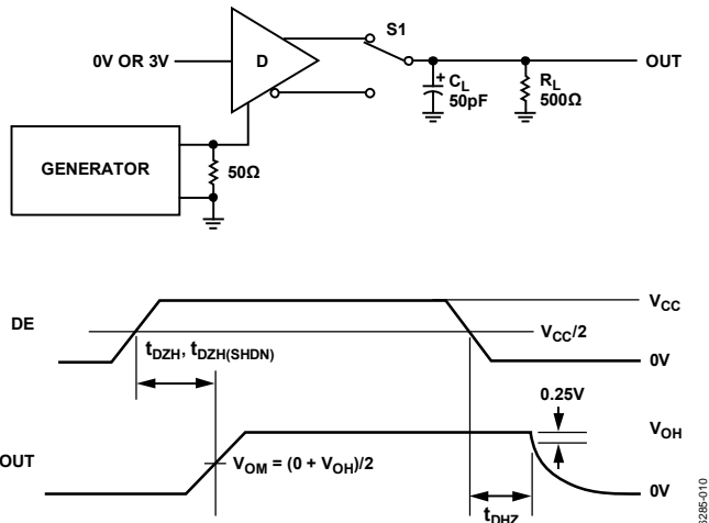
Figure 10. Driver Enable and Disable Times ( t_{DZH} , t_{DZH(SHDN)} , t_{DZL} )
