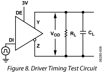
Figure 8. Driver Timing Test Circuit
