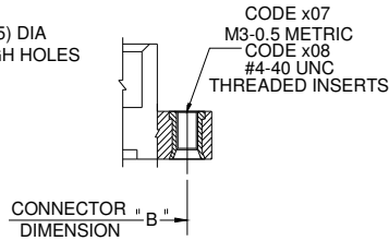
CONNECTOR "B" DIMENSION MOUNTING OPTION CODES x07 & x08 (THREADED INSERTS)
