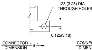
CONNECTOR "B" DIMENSION MOUNTING OPTION CODE x12 (SIDE MOUNTING HOLES) WITH INSERTS: CODES x17 & x18, SEE TABLE
