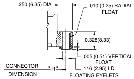
CONNECTOR "B" DIMENSION MOUNTING OPTION CODE x03 (FLOATING EYELETS)
