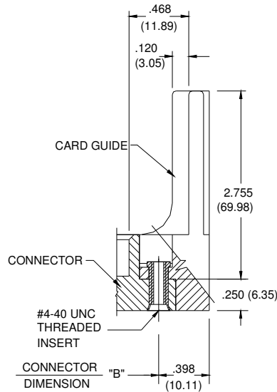
CONNECTOR "B" DIMENSION MOUNTING OPTION CODES x58 (OFFSET CARD GUIDES)
