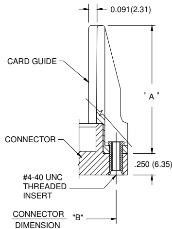
CONNECTOR "B" DIMENSION MOUNTING OPTION CODE x78 (IN-LINE CARD GUIDE)
