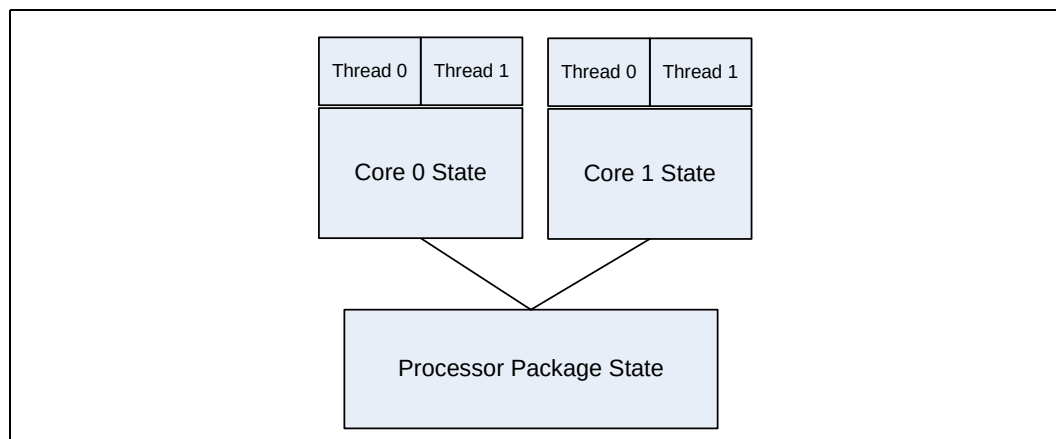
Figure 6-2. Idle Power Management Breakdown of the Processor Cores
