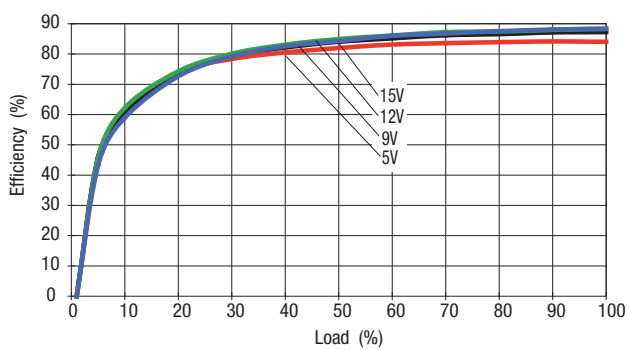
MTU1x12xxMC
