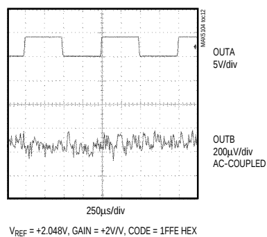
ANALOG CROSSTALK
