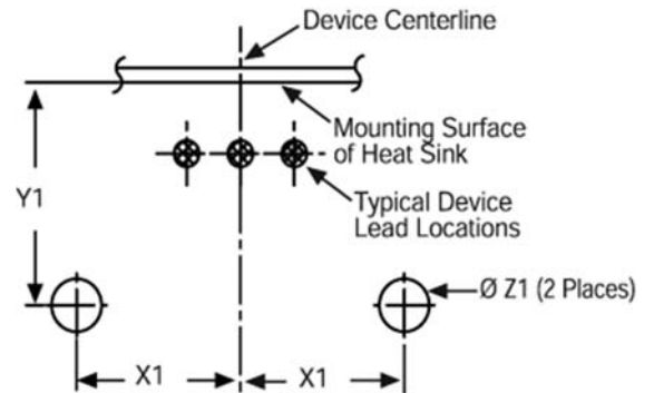
Mounting Details:
