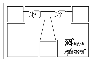
MA4E1319 - 2
