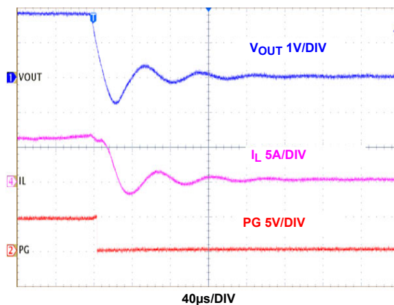
FIGURE 30. OVERCURRENT PROTECTION
