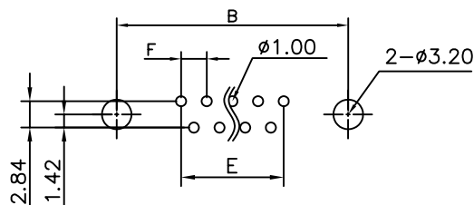
RECOMMENDED P.C.B LAYOUT (TOLERANCE \pm 0.03 )
