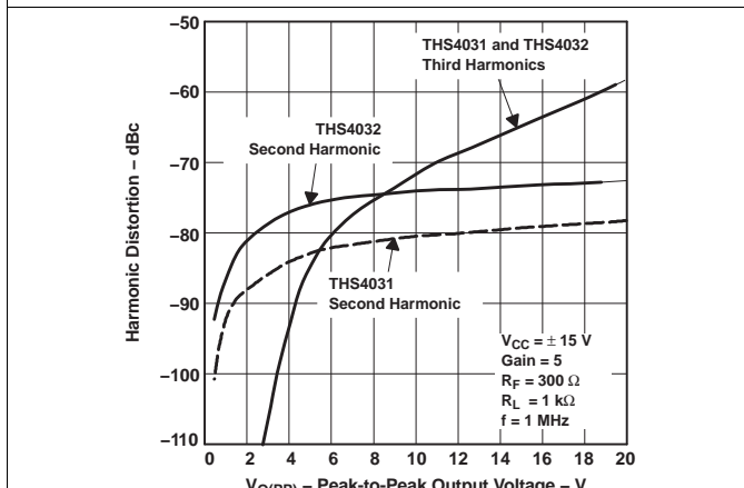
Figure 17. Harmonic Distortion vs Peak-to-Peak Output Voltage
