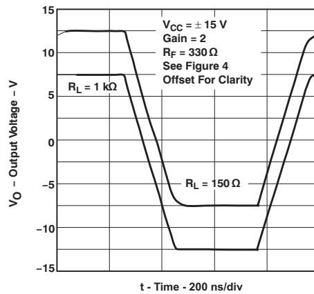
Figure 45. 20-V Step Response
