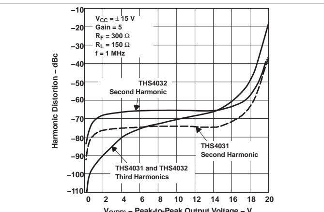
Figure 18. Harmonic Distortion vs Peak-to-Peak Output Voltage
