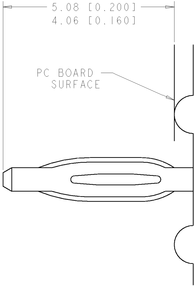
5. COMPLIANT PIN DETAIL SCALE 10 : 1 INSERTION/EXTRACTION FORCES MAXIMUM PUSH IN: 133.3N PER PIN (30 LBS) MINIMUM PUSH OUT: 44.4N PER PIN (10 LBS)
