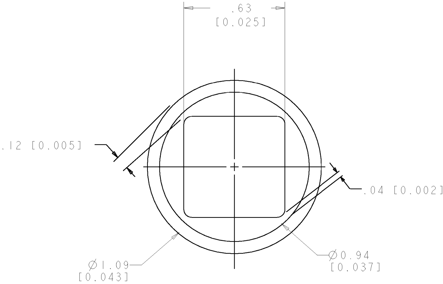
6. SOLDER TERMINATION AREA SCALE 40:1 RECOMMENDED PRINTED CIRCUIT SOLDER HOLE DRILLED HOLE: Ø1.15 [0.0453] ±.013 [0.0005] COPPER PLATE: .025 [0.0010] MIN TIN PLATE: .008 [0.0003] MIN. (PER SURFACE)
