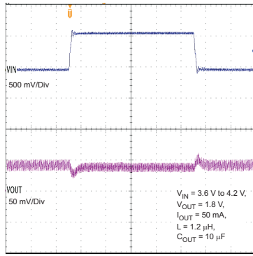
Time Base - 100 \mu s/Div Figure 21. Line Transient PFM Mode
