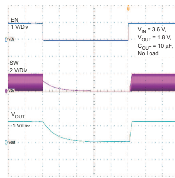
Time Base - 2ms/Div Figure 23. Output Discharge
