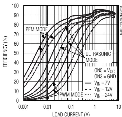
MAX8733A 5V OUTPUT EFFICIENCY vs. LOAD CURRENT
