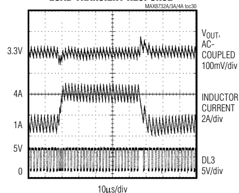
MAX8733A/MAX8734A (TON = GND) 3.3V PWM-MODE LOAD TRANSIENT RESPONSE
