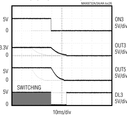
SHUTDOWN WAVEFORMS
