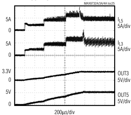
SOFT-START WAVEFORMS
