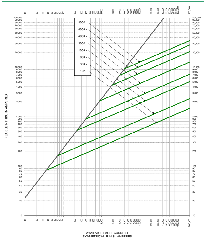
Peak Let-Thru Curve
