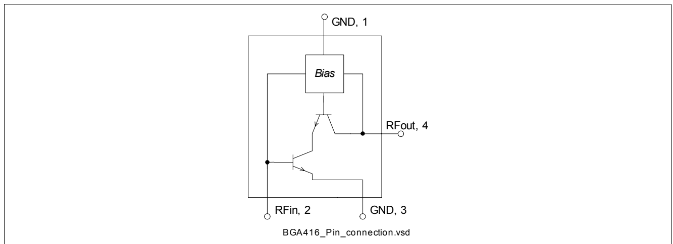
Figure 1 Pin connection
