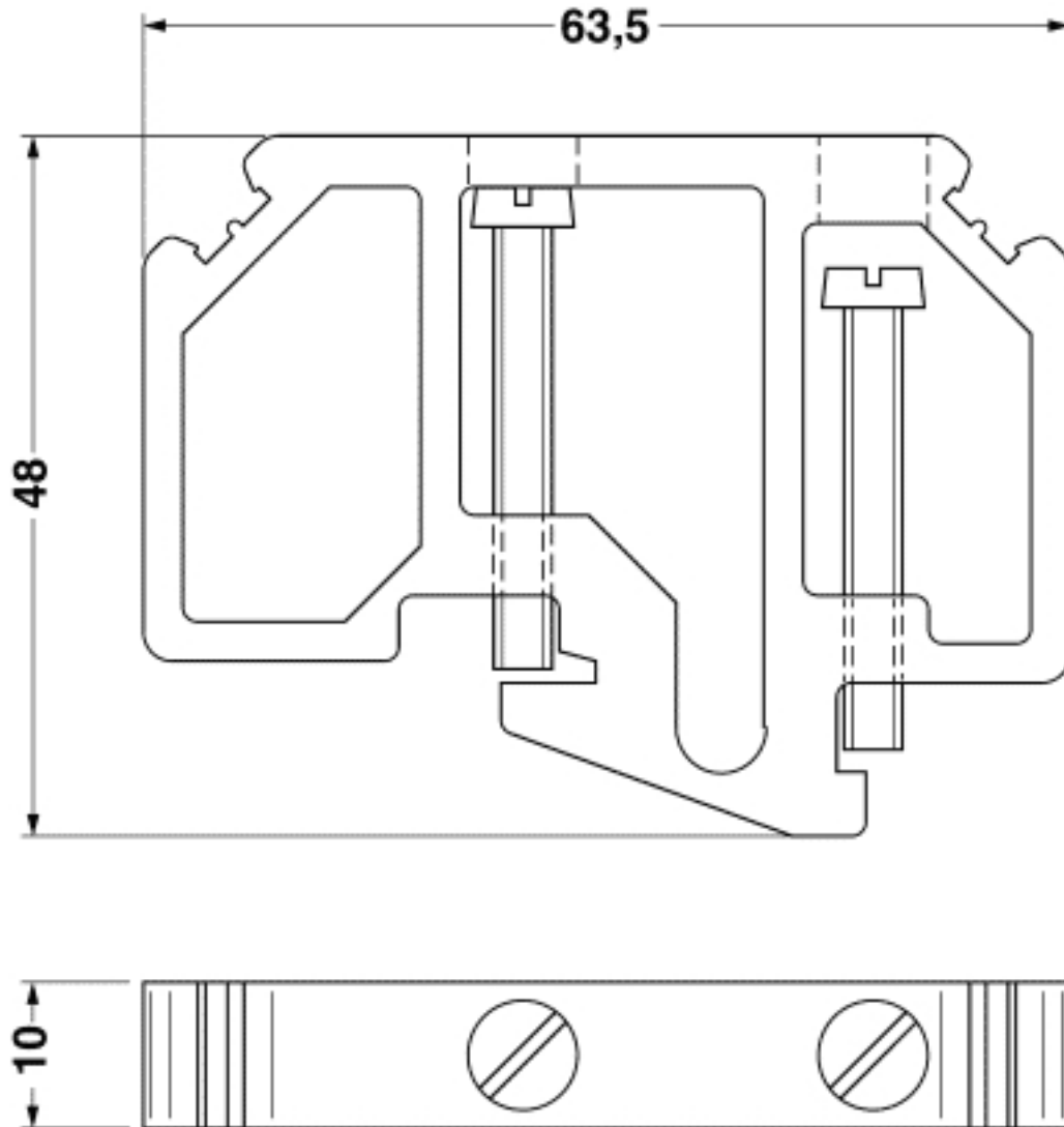
Dimensional drawing
