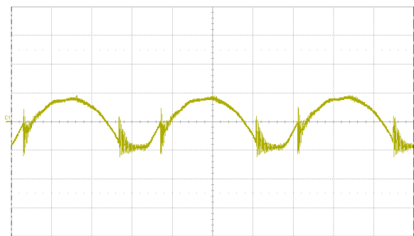
Fig. 13: Output voltage ripple (20 mV/div.) at full rated load current into a resistive load with C_o = 10\ \mu\text{F} tantalum + 1\ \mu\text{F} ceramic and V_{in} = 48\ \text{V} . Time scale: 1\ \mu\text{s}/\text{div} .
