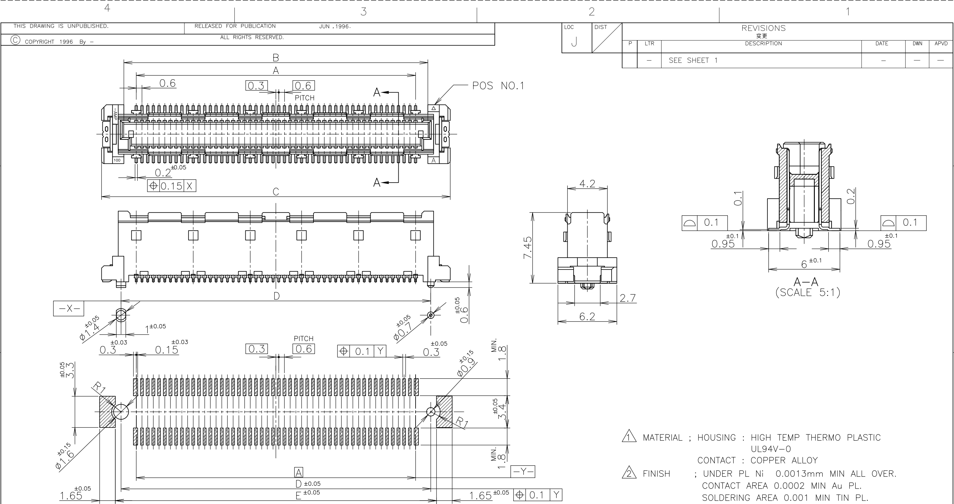
REFERENCE P.C.BOARD LAYOUT (VIEW FROM CONN. MOUNTING SIDE)
