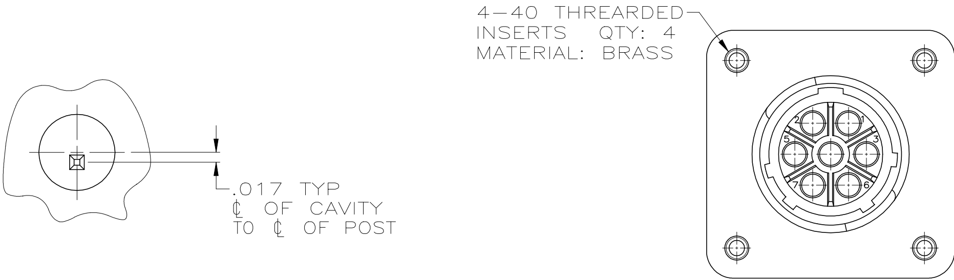
POST ARRANGEMENT ON REAR FACE SCALE 6:1
