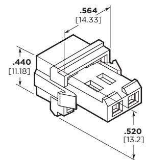
Two-Position Only 641533-1
