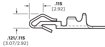
A High Force (6.5 Amp Max. Current Rating)
