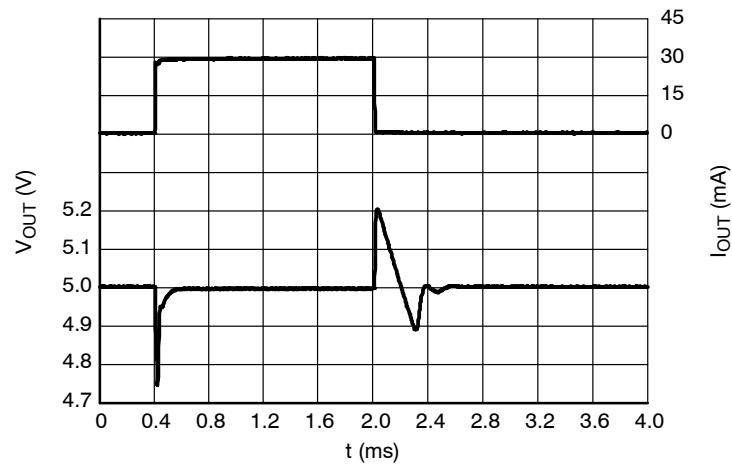
Figure 61. Load Transients, 5.0 V Version, I_{OUT} = 1 - 30 \text{ mA} , t_R = t_F = 0.5 \text{ } \mu\text{s} , V_{IN} = 8.0 \text{ V} , ECO = L
