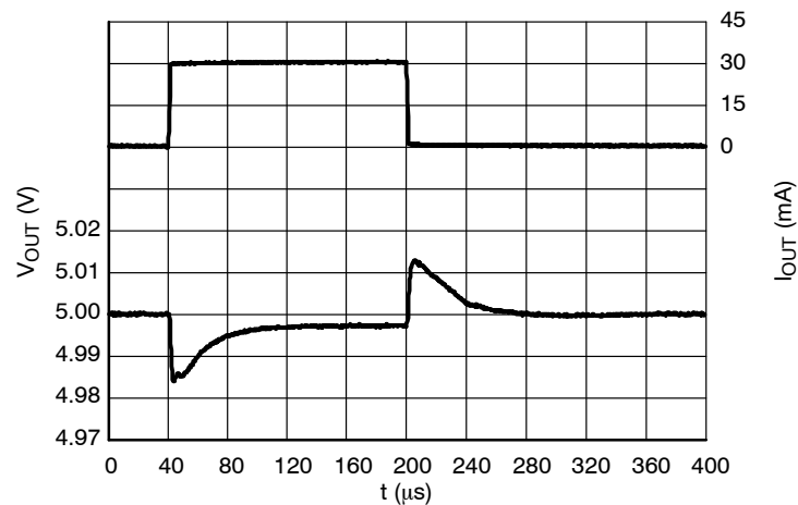
Figure 62. Load Transients, 5.0 V Version, I_{OUT} = 1 - 30 \text{ mA} , t_R = t_F = 0.5 \text{ } \mu\text{s} , V_{IN} = 8.0 \text{ V} , ECO = H
