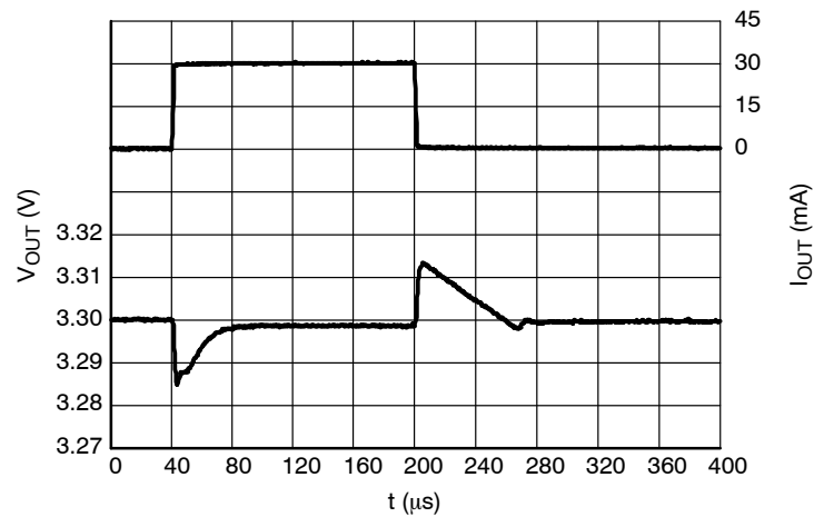
Figure 60. Load Transients, 3.3 V Version, I_{OUT} = 1 - 30 \text{ mA} , t_R = t_F = 0.5 \text{ } \mu\text{s} , V_{IN} = 6.3 \text{ V} , ECO = H
