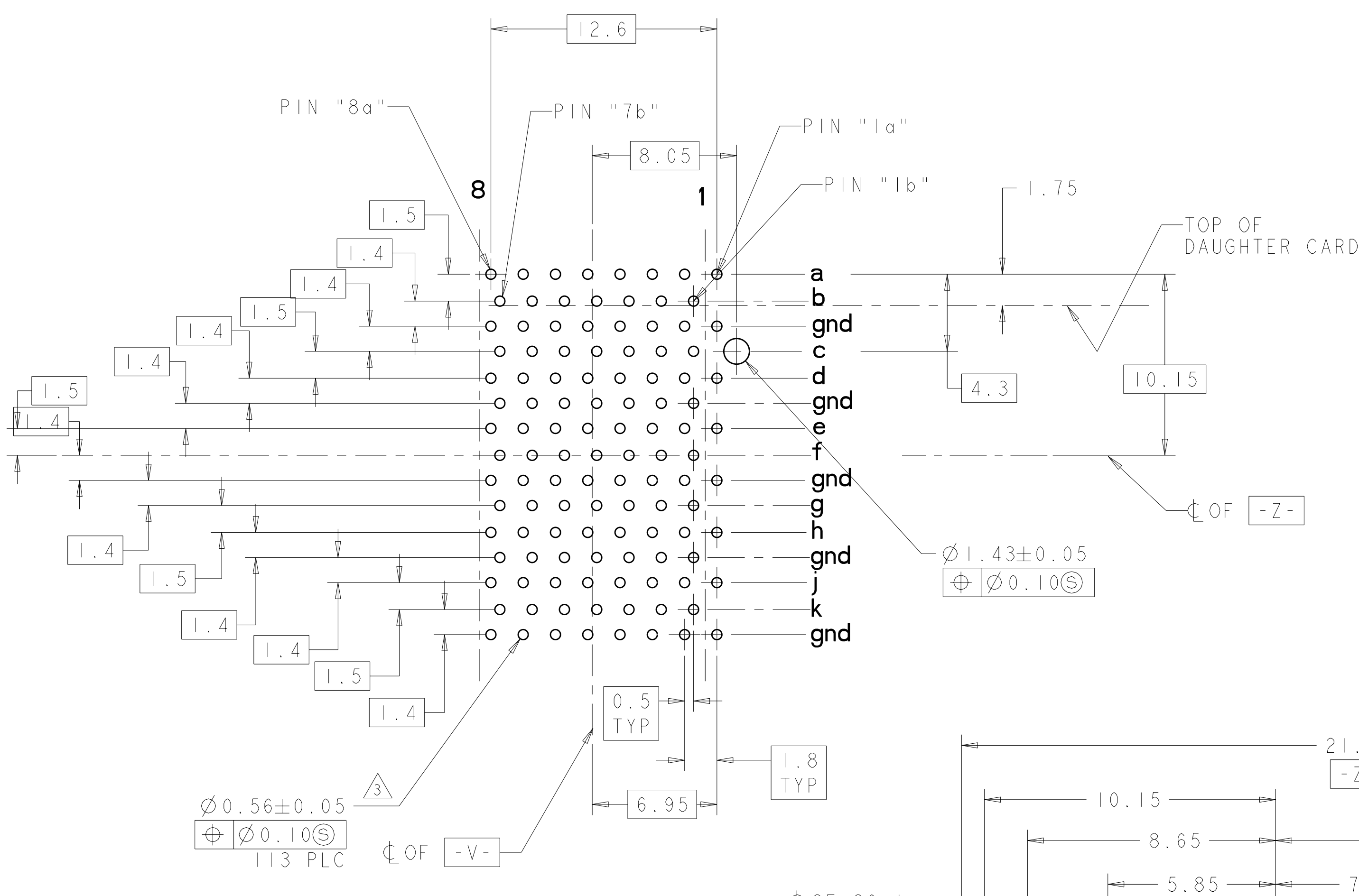
PC BOARD FOOTPRINT VIEWED FROM CONNECTOR SIDE SCALE 5:1
