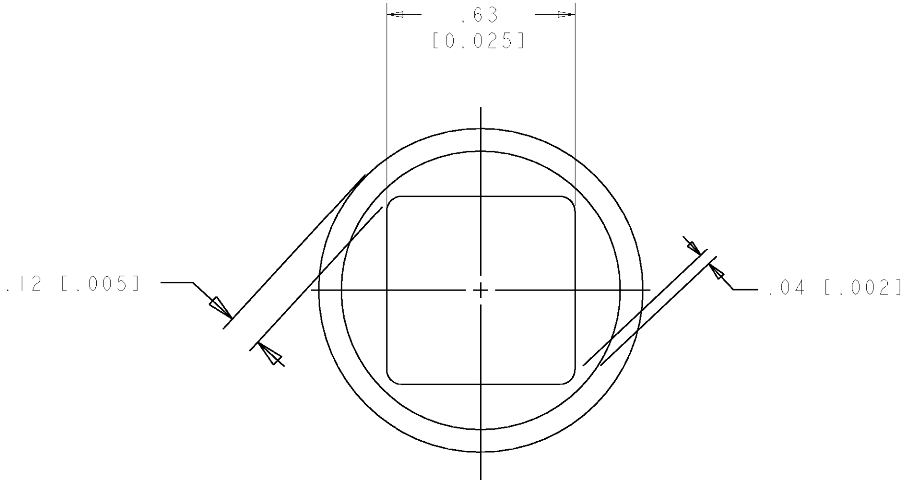
9. SOLDER TERMINATION AREA SCALE 40:1 RECOMMENDED PRINTED CIRCUIT SOLDER HOLE FINISHED HOLE: \varnothing 1.02 [.040] \pm .08 [.003] DRILLED HOLE: \varnothing 1.15 [.0453] \pm .013 [.0005] COPPER PLATE: .025 [.0010] MIN TIN PLATE: .008 [.0003] MIN. (PER SURFACE)
