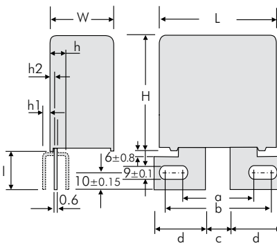
2-pin version
