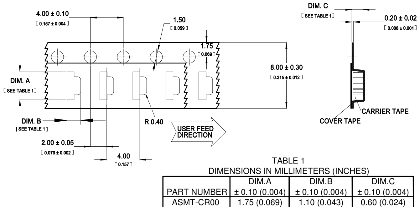
Figure 11. Tape dimensions.
