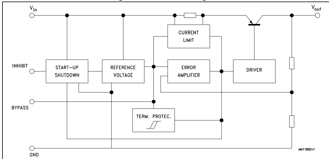
Figure 1. Schematic diagram
