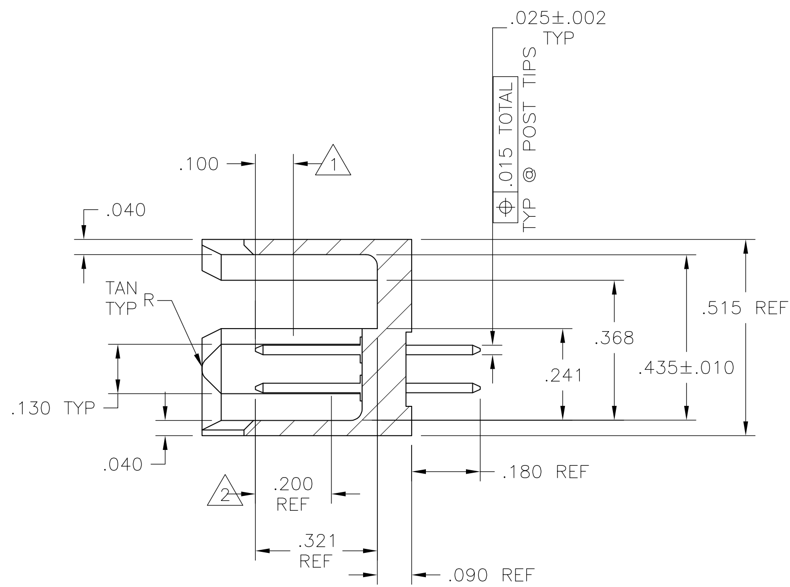
SECTION X-X
