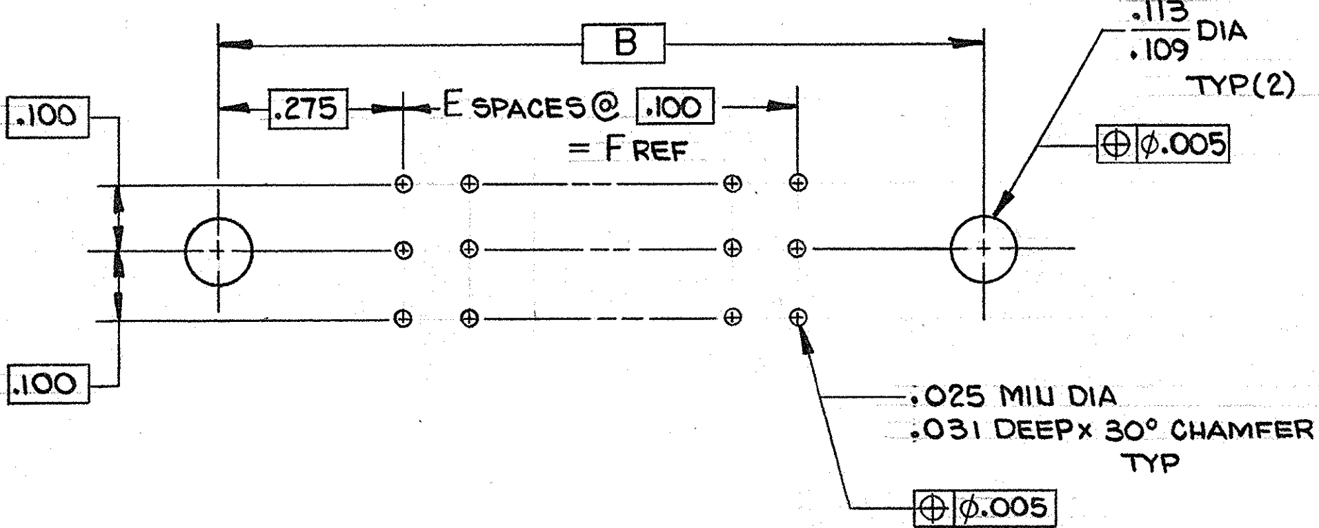
P.C. BOARD LAYOUT
