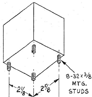
STUD MOUNTING MODEL 710 MODELS 720 THRU 724
