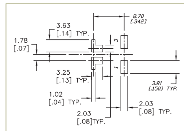
P.C. MOUNTING
