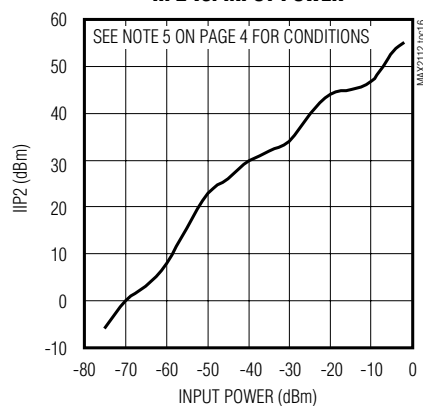
IIP2 vs. INPUT POWER
