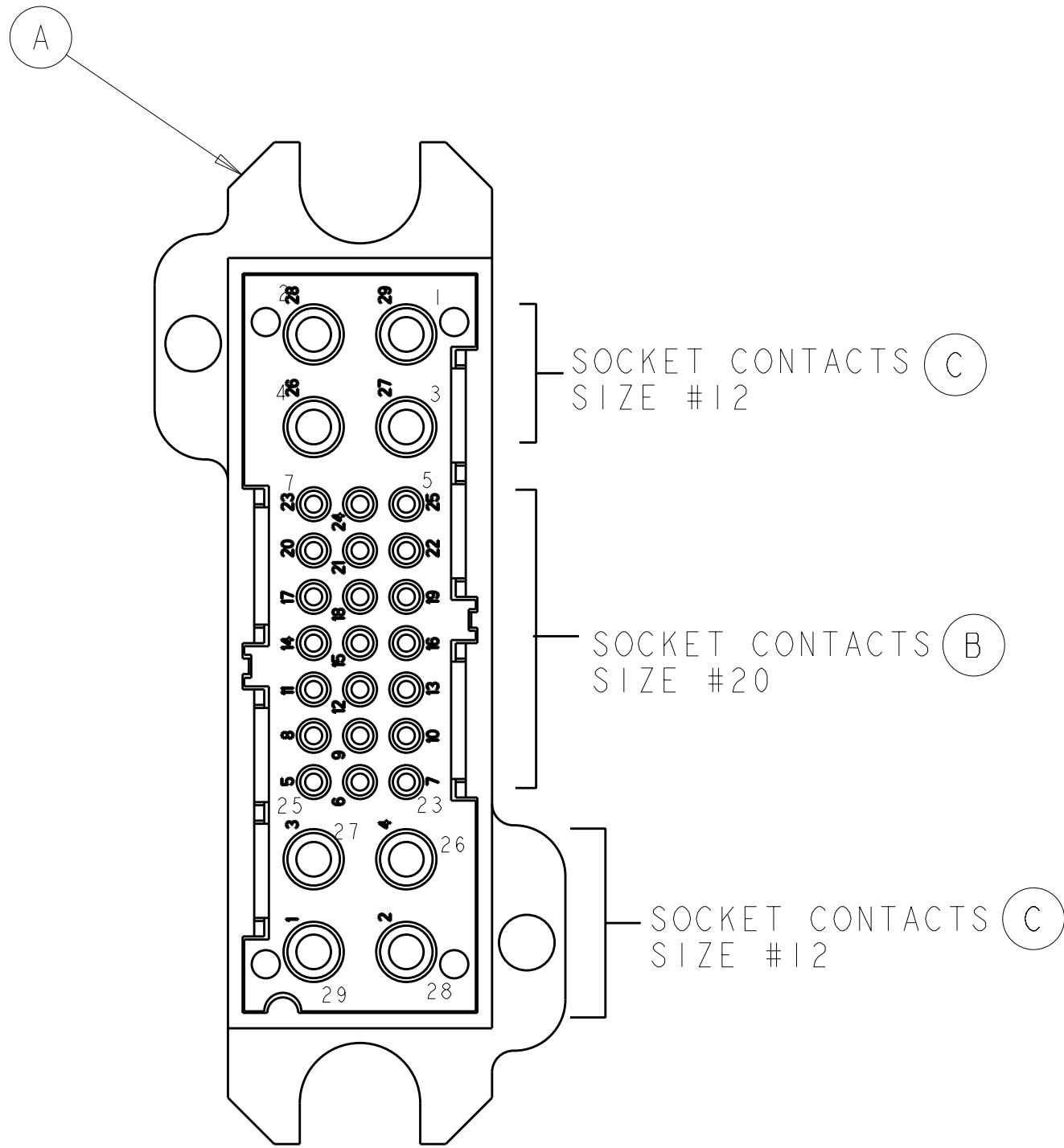
REAR VIEW
